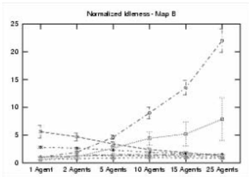
Fig. 6. Graph Normalized Idleness for Map B.
